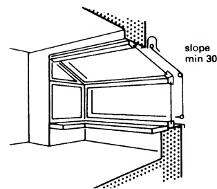
⑥ Sloping awning with vertical fringe
